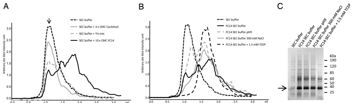
Fig. 3. Size-exclusion chromatography analysis of hOR17-4 aggregation states. (A) We used Superdex 200 GL 5/150. SEC analysis in different detergents, running buffer: SEC buffer [25 mM Tris-HCl (pH 7), 150 mM NaCl, 10% glycerol] supplemented with 3× CMC cyclofos 5 (gray line), Tri-mix (gray dashed line), 10× CMC FC14 (black line), and SEC buffer only (black dotted line). The arrow indicates the void volume. (B) Monitoring the effect of hOR17-4 aggregation states in different buffers with different pH, NaCl concentration, and reducing agent. (C) SDS/PAGE of the elution fractions from affinity purification with the same buffers as in B.
