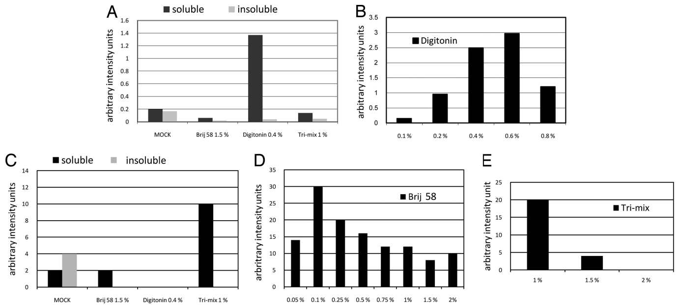
Fig. 2. The effects of additional screen of different detergents on olfactory receptor production levels in wheat germ cell-free production system. The amount of soluble (black bars) and insoluble (gray bars) produced mOR23 (A) and mS51 olfactory receptor production (C) with Brij58, digitonin, and Tri-mix. Titration of detergent concentration for production of soluble mOR23 (B) and mS51 (D and E).
